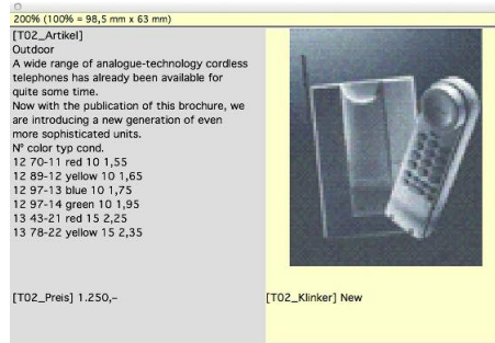
in DATAform 11
